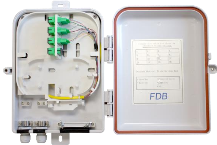
16 port
